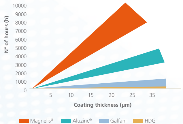
N° of hours before appearance of 5% red rust
