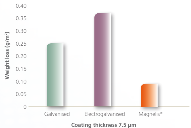
Lubrication: Fuchs 4107S in excess Powdering behaviour comparison between metallic substrates expressed in weight loss (g/m 2 )
